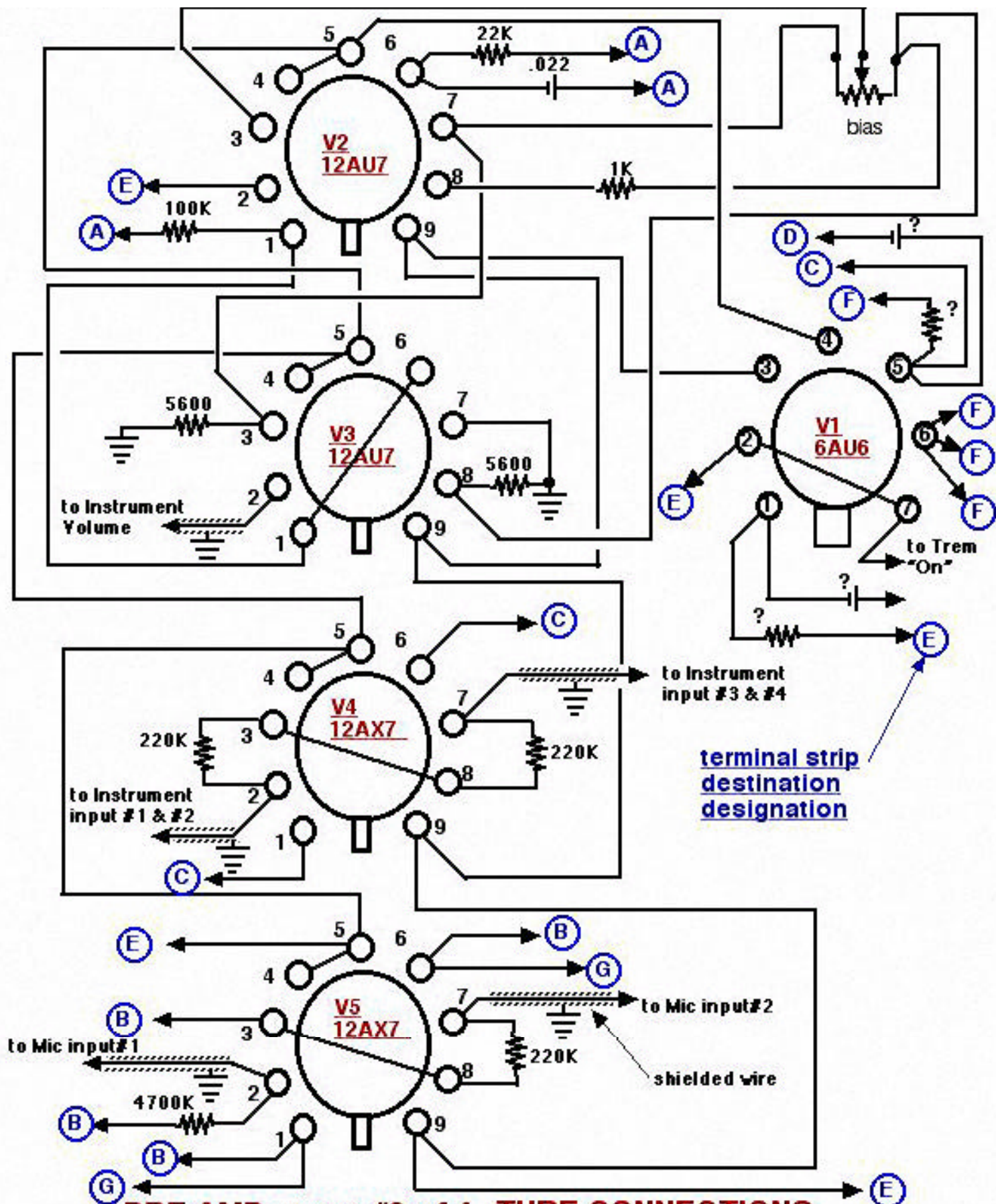
PRE AMP page #2 of 4 TUBE CONNECTIONS
