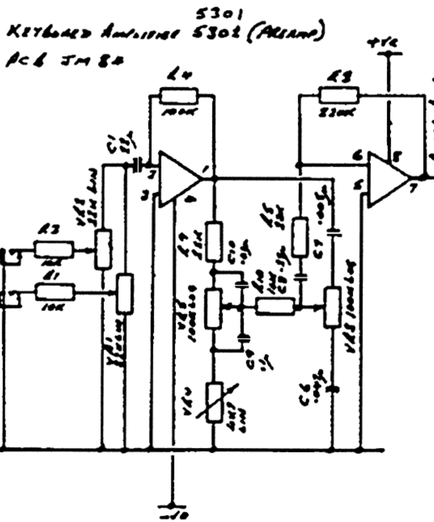
MARSHALL 20Watt Combo Series 5002, 5302, 5502. Circuit Diagram. 30-3-84 12 Watt Keyboard Combo 5301 1552 6-6-86 R.S.
