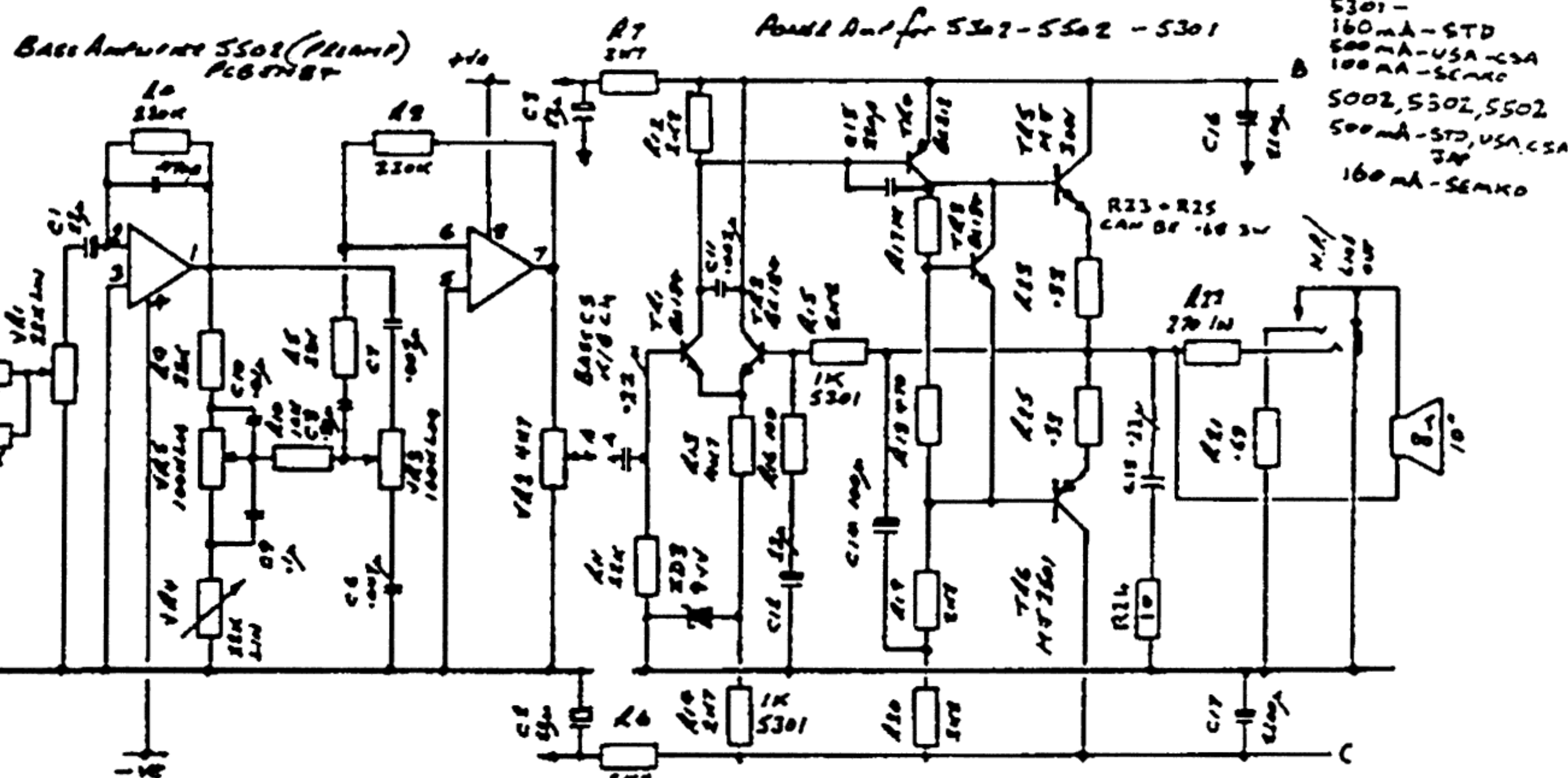
MARSHALL 20Watt Combo Series 5002, 5302, 5502. Circuit Diagram. 30-3-84 12 Watt Keyboard Combo 5301 1552 6-6-86 R.S.
